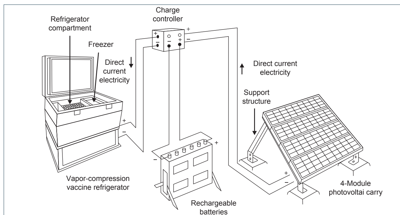
Figure 14: Solar Refrigeration System
