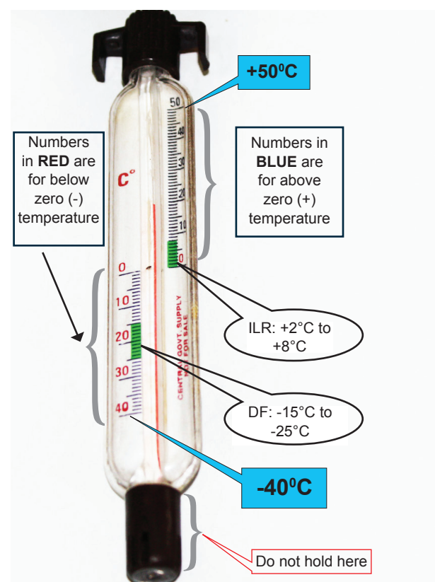
Alcohol Stem Thermometer
